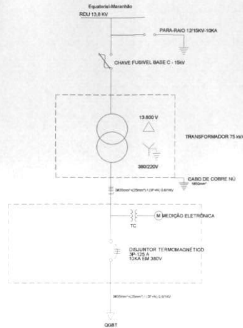
DIAGRAMA UNIFILAR
